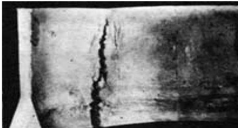
Fig Hot tears in part
